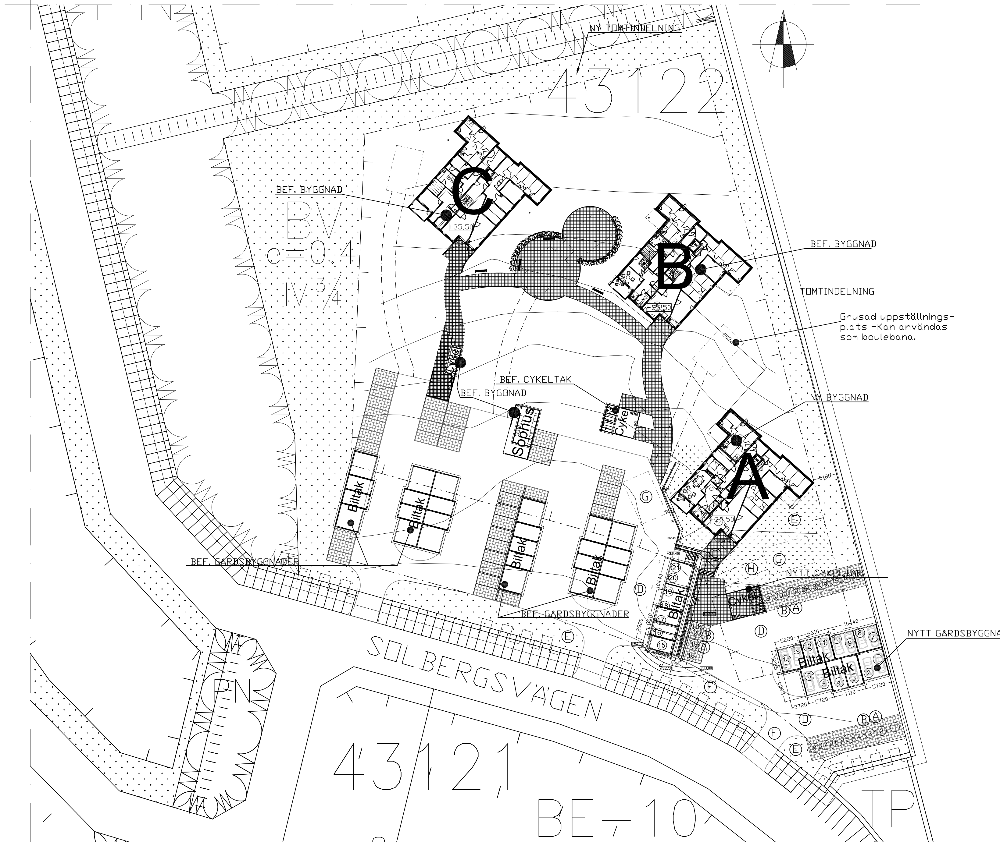
Situationsplan Skala 1:500
